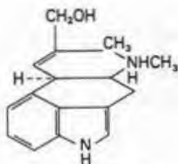
CHANOCLAVINE
